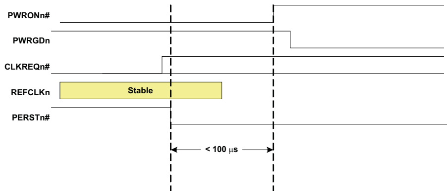
Figure 5-4. Normal Power-Down
