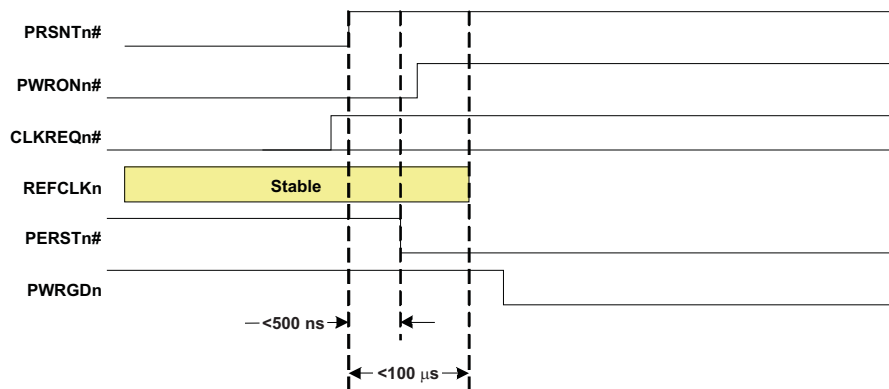
Figure 5-5. Surprise Removal
