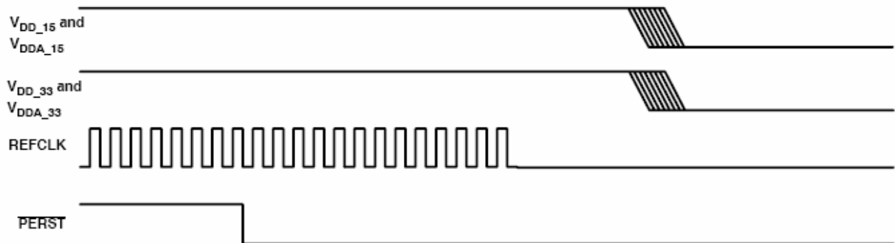
Figure 3-3. Power-Down Sequence Diagram
